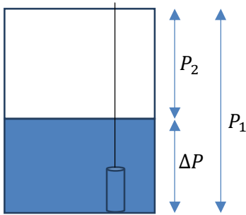
Gambar 2. Sistem Differential Pressure Level Sensor
